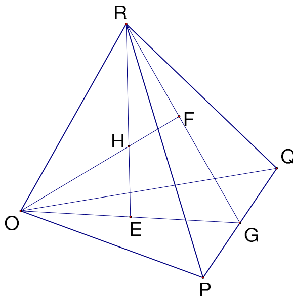
Figure 2: Regular tetrahedron
