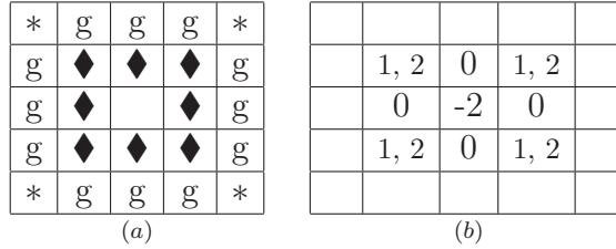
FIGURE 12. Local Configuration Near a Guard with Deficiency -2
