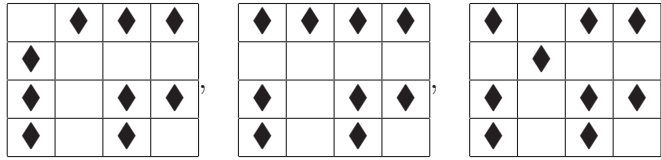
FIGURE 4. Maximum 4 \times 4 Boards
